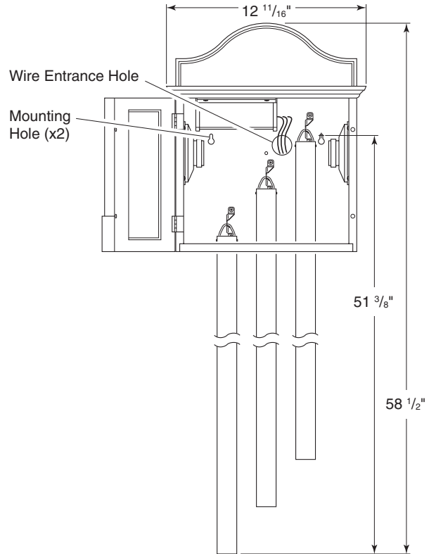
Figure 1 - Chime Dimensions
